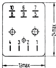
V23154-C0xx, size I type
