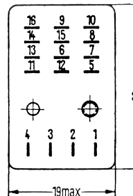
V23162-B0xx, size II type V23162-H0xx, size II type
