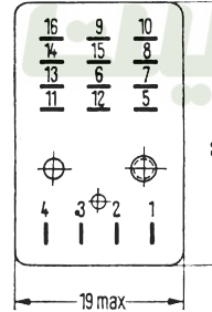
V23154-D0xx, size II type
